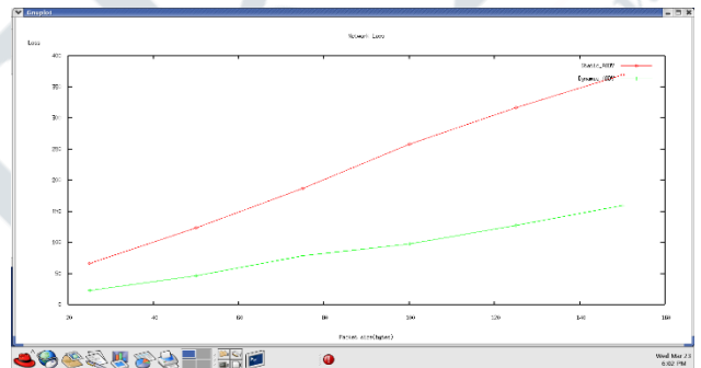
Fig.1.9 Network loss for static and dynamic AODV
