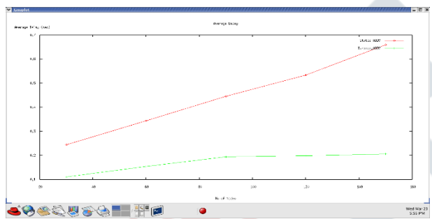
Fig.1.7 Average delay for static and dynamic AODV
